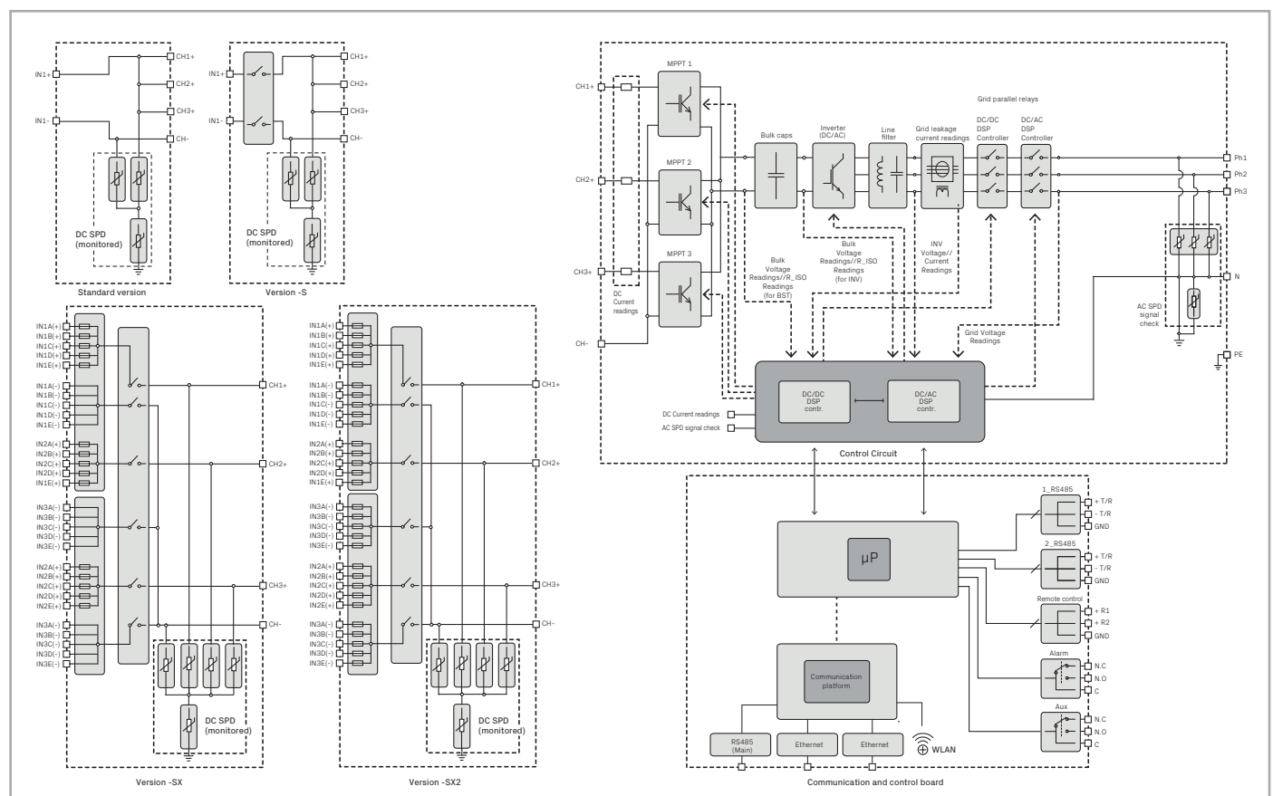
PVS-50/60-TL string inverter block diagram
