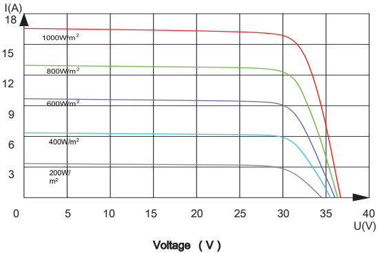
Current-Voltage Curve (470W)
